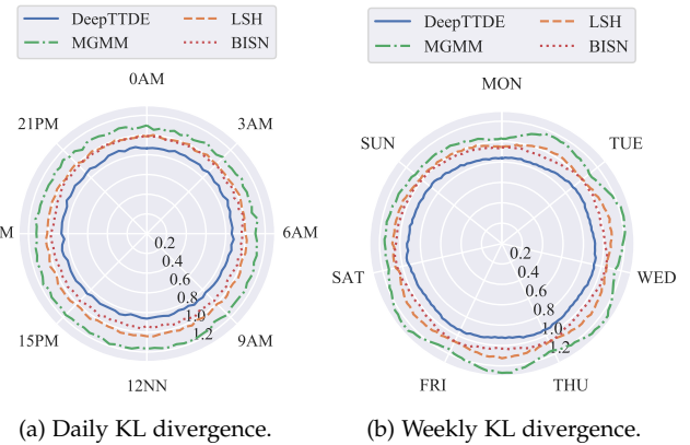
Fig. 3. KL divergence performance of DeepTTDE and best-performing baselines.
