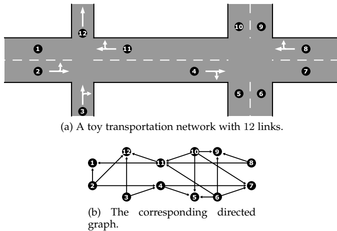
Fig. 1. An example of the graph representation of transportation network.
